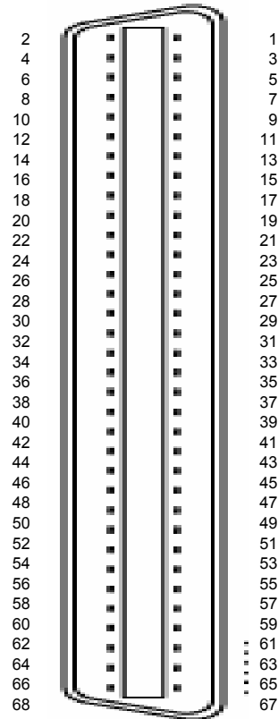
Front View of Connector
